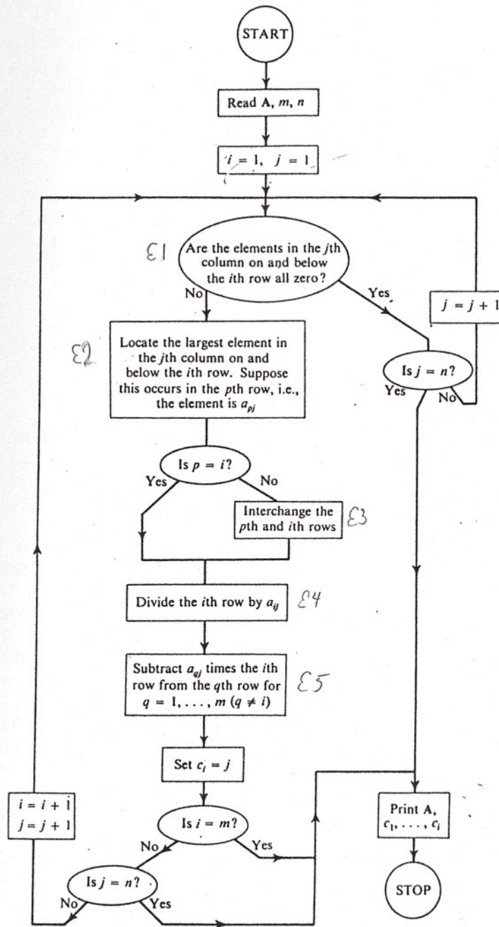
Figure 3.2 Flow-chart for row-echelon form.
