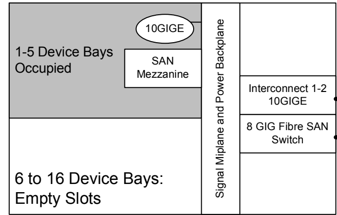
Simplified Side View of HP C7000 Chassis
