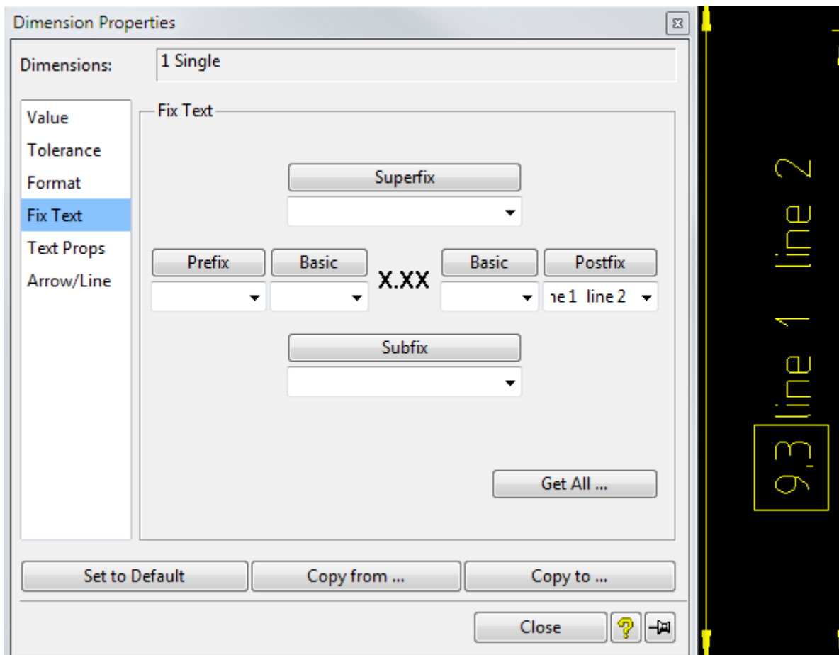
Picture 3: It is not possible to add a multiline Postfix to a Dimension with Tolerance Type "Basic"
